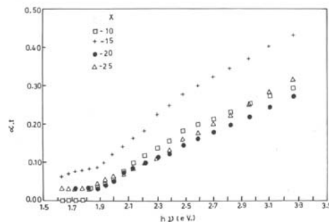
Fig.2 Variation of \alpha.t as a function of photon energy in annealed thin films of \text{Te}_5(\text{In}_x\text{Se}_{100-x})_{95} glassy alloys
