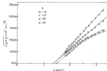
Fig. 6 Variation of (ahv)^{1/2} versus hv in annealed thin films of Te_5(In_xSe_{100-x})_{95} glassy alloys; the solid lines represent the least square fit.
