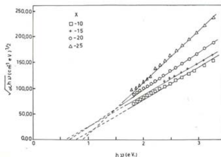
Fig. 5 Variation of (ahv)^{1/2} versus hv in as-prepared thin films of Te_5(In_xSe_{100-x})_{95} glassy alloys; the solid lines represent the least square fit.
