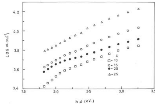
Fig. 3. Variation of the absorption coefficient ( \text{Log} \alpha ) with energy in as-prepared thin films of \text{Te}_5(\text{In}_x\text{Se}_{100-x})_{95} glassy alloys
