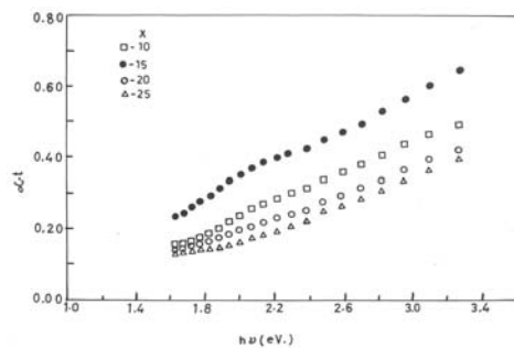
Fig.1 Variation of \alpha.t as a function of photon energy in as-prepared thin films of \text{Te}_5(\text{In}_x\text{Se}_{100-x})_{95} glassy alloys
