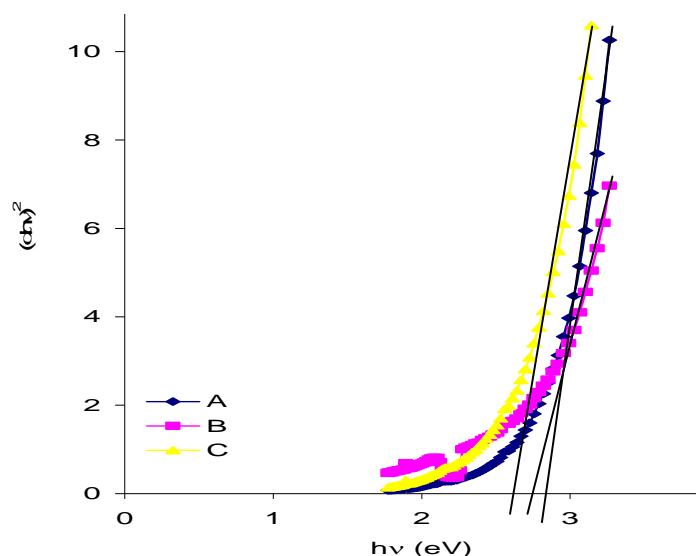
Fig.7: (ahv)^2 vs. h\nu for lead oxide thin films.
