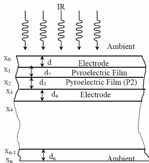
Fig. 1. A cross section of an n-layer detector structure.
