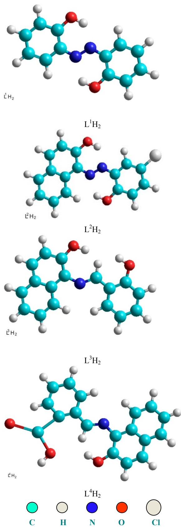
Fig. 1 The chemical structures of ligands
