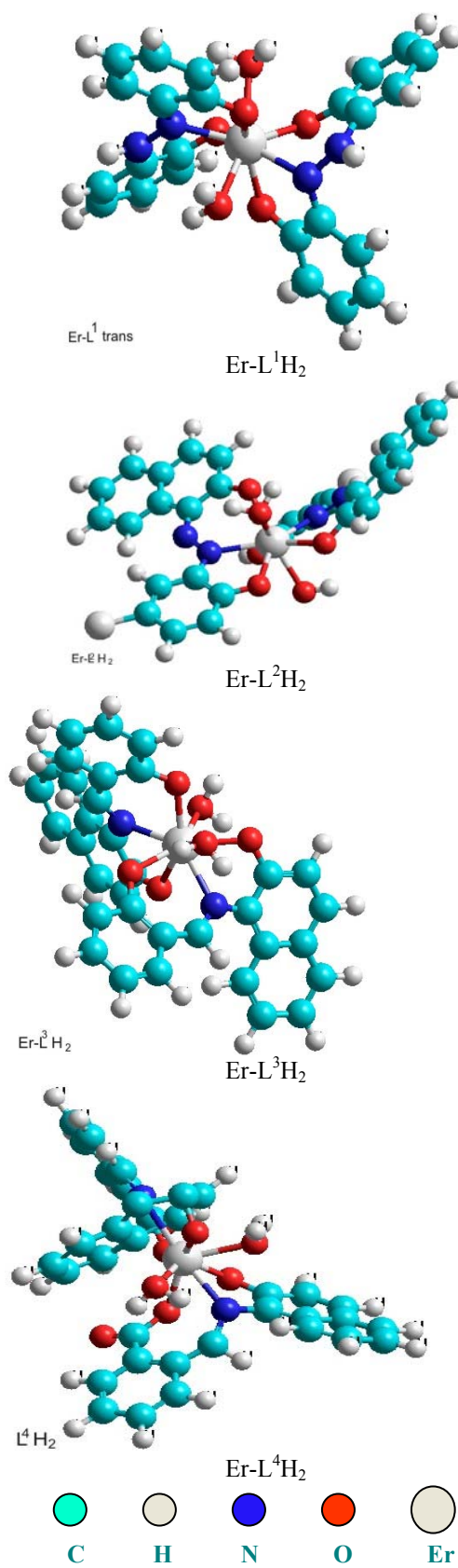
Fig. 2 The chemical structures of Er-ligands complexes
