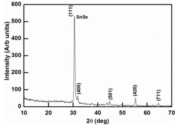
Fig. 1 XRD pattern of the SnSe thin film.
