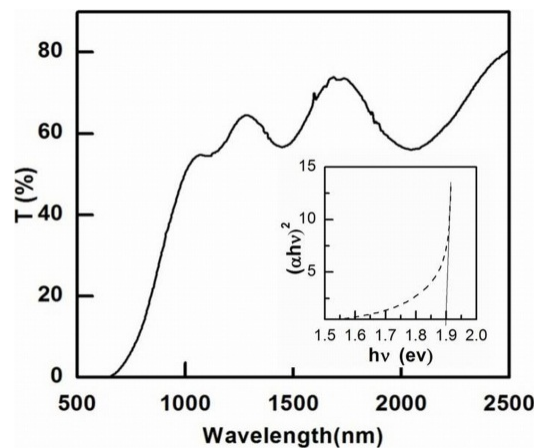
Fig. 2 Optical transmission spectrum of the SnSe thin films. Inset shows the bandgap of the film (1.9 eV).
