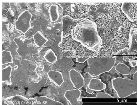
Fig. 3 SEM micrograph of the SnSe thin films the inset shows the inter grain space.
