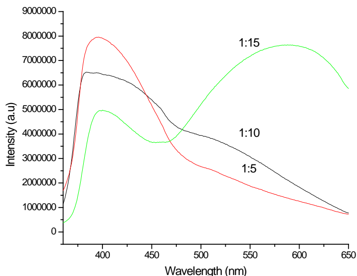
Fig.5 Room temperature Photoluminescence spectra obtained at three different growth solution concentrations
