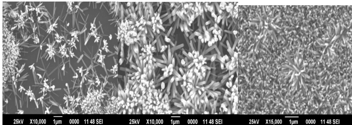
Fig.2 SEM images of nano rods grown on different growth solution concentration of 1:5, 1:10 & 1:15
