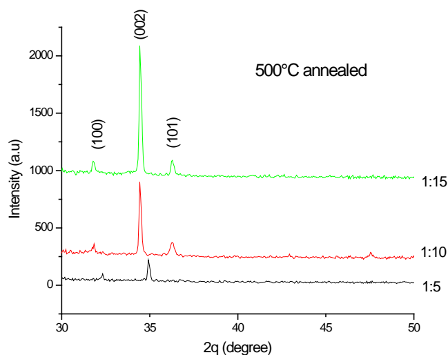
Fig.1 XRD pattern of ZnO nano rod array at three different growth concentrations
