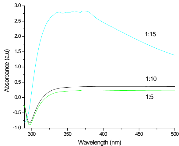
Fig.3 Absorption spectra obtained at three different growth solution concentrations
