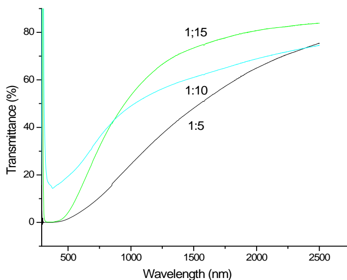
Fig.4 Transmittance spectra obtained at three different growth solution concentrations
