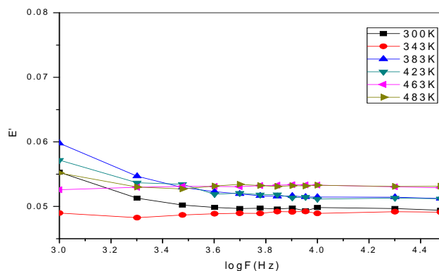
Fig. 3. Variation of Dielectric constant \epsilon' with log frequency at different temperatures for PbSe thin film of thickness 2000 Å
