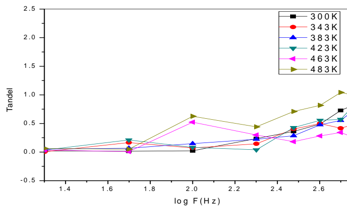
Fig. 2. Variation of \tan\delta with log frequency at different Temperatures for PbSe thin film of thickness 1000 Å.
