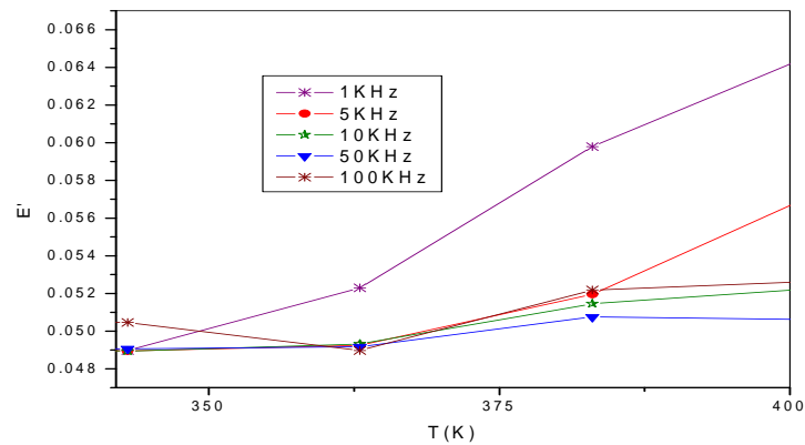
Fig. 5. Temperature dependence of permittivity at different Frequencies for PbSe thin film of thickness 1000 Å
