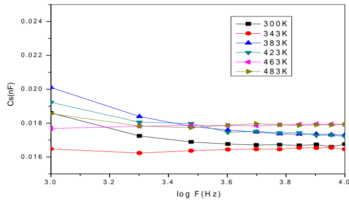
Fig. 1. Variation of capacitance C_s with log frequency at different temperatures for PbSe Thin film of thickness 1000 Å
