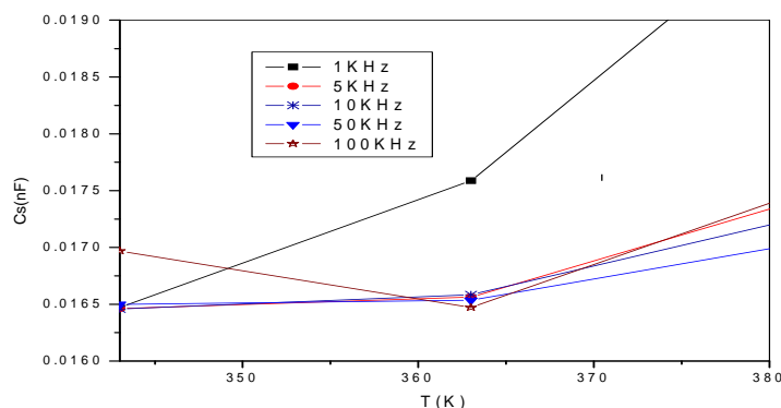
Fig. 4. Temperature dependence of capacitance at different Frequencies for PbSe thin film of thickness 1000 Å
