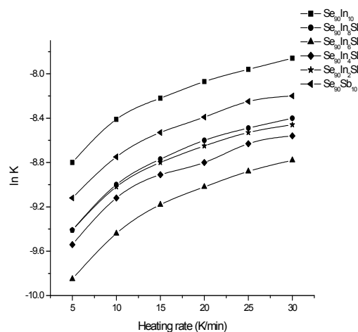
Fig. 5(b): Plot of \ln K versus heating rate at different Sb concentration
