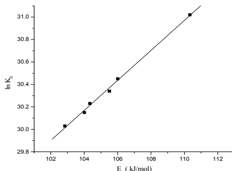
Fig. 6: The plots of \ln K_0 vs. E_c for glassy \text{Se}_{90}\text{In}_{10-x}\text{Sb}_x systems
