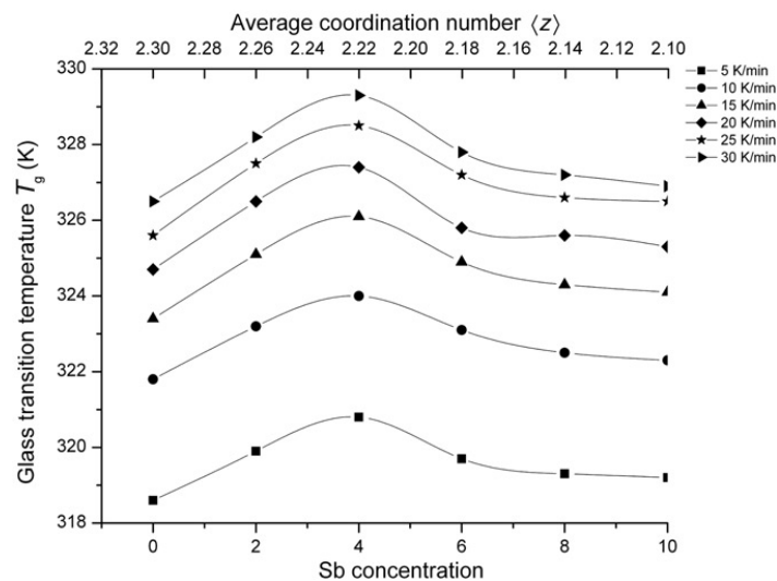
Fig. 3: Variation in glass transition temperature T_g with Sb concentration and average coordination number \langle z \rangle at different heating rates.
