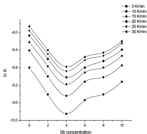
Fig. 5(a): Plot of \ln K versus Sb concentration at different heating rates
