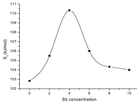
Fig. 4 Plot of activation energy E_c versus Sb concentration
