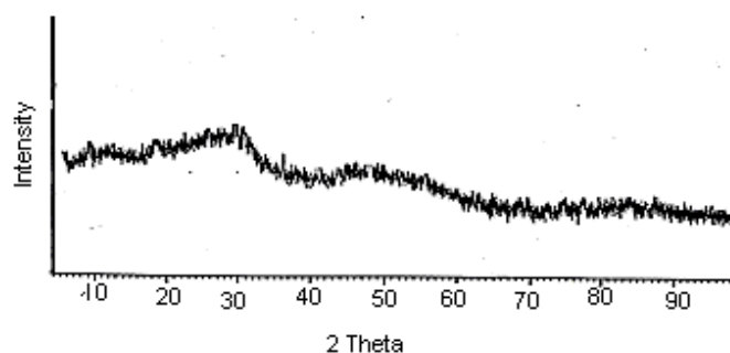
Fig.1: XRD pattern of \text{Se}_{90}\text{In}_8\text{Sb}_2 chalcogenide glass at room temperature in powder form
