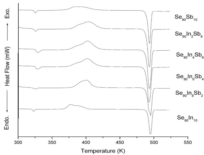
Fig. 2: DSC traces of Se_{90}In_{10-x}Sb_x ( x=0, 2, 4, 6, 8, 10 ) chalcogenide glass at a heating rate of 10 K/min heating rate.
