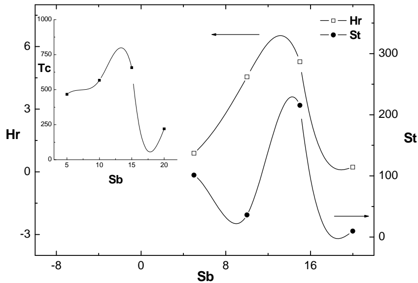
Fig. 4. Composition dependence of thermal stability parameters ( s ), Hurby number ( Hr ), and crystallization temperature
