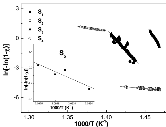
Fig. 3. Plot of \ln[-\ln(1-\alpha)] versus 1/T for investigated samples.
