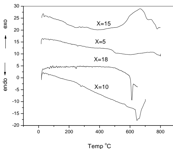
Fig. 1. DTA themograms obtained at heating rate 10^\circ\text{C}/\text{min}
