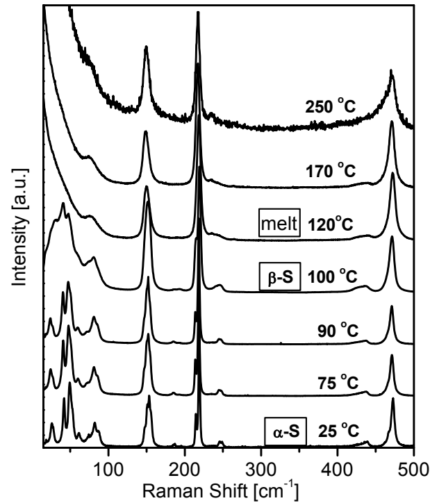
Fig. 2 Temperature dependence of Raman spectra of distilled sulfur.
