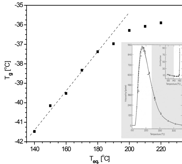
Fig. 3 Dependence of glass transition temperature on melt equilibrium temperature T_{eq} , see text. Inset: Temperature dependence of sulfur viscosity [9]. White areas cover experimental temperatures.
