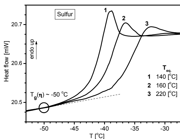
Fig. 4 Example of width of the glass transition region broadening when melt equilibrium temperature T_{eq} increases. Viscosity glass transition is also indicated.
