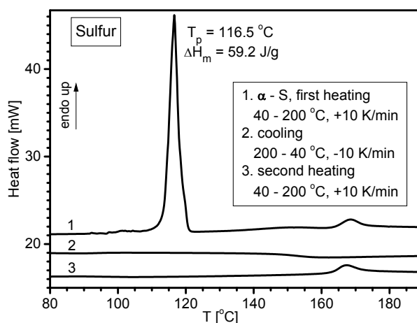
Fig. 1 Set of conventional DSC scans starting with \alpha -sulfur. For more details, see text.
