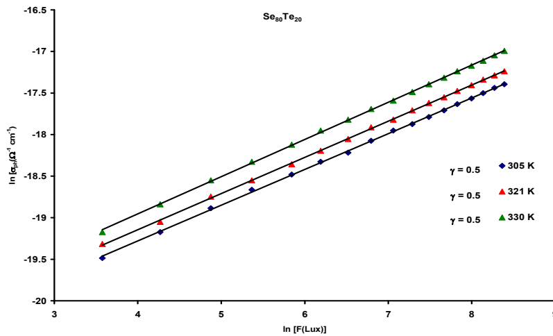
Fig. 3. Intensity dependence of photoconductivity at various temperatures in a\text{-Se}_{80}\text{Te}_{20} .
