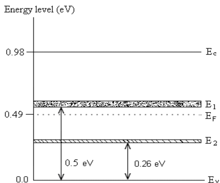
Fig. 5. Energy level diagram for defect states in the mobility gap of a-Se 80 Te 10 Cd 10 thin films at a particular intensity of light 1190 Lux.
