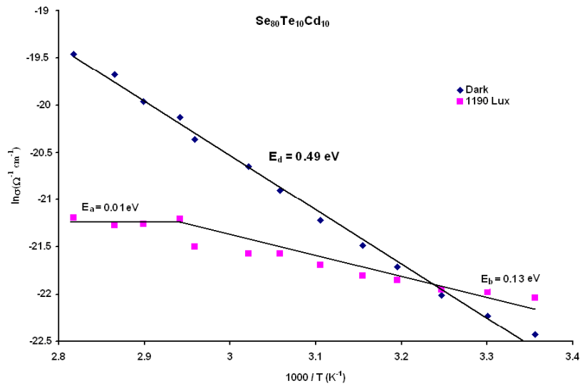
Fig. 2. Temperature dependence of photoconductivity in amorphous thin films of a-Se_{80}Te_{10}Cd_{10} at a intensity of 1190 Lux.
