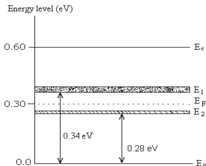
Fig. 4. Energy level diagram for defect states in the mobility gap of a- Se_{80}Te_{20} thin films at intensity of light 559 Lux.
