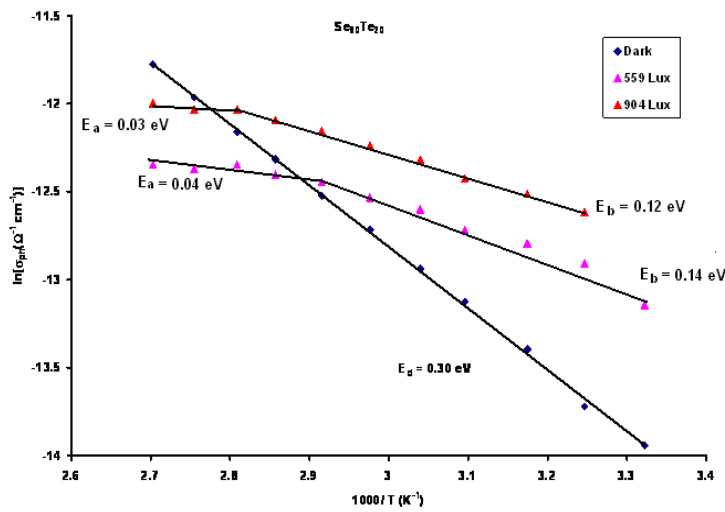
Fig. 1. Temperature dependence of photoconductivity in amorphous thin films of Se_{80}Te_{20} at intensities of 559 lux and 904 lux.
